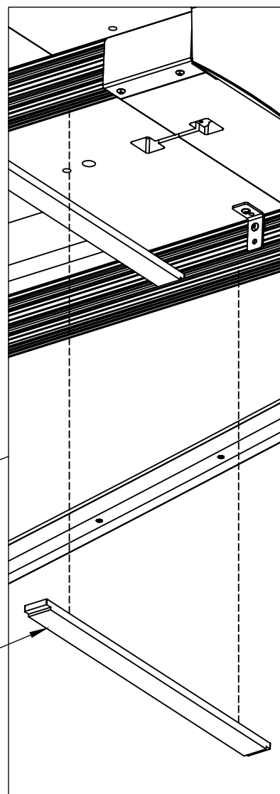
Wire Management Slat
