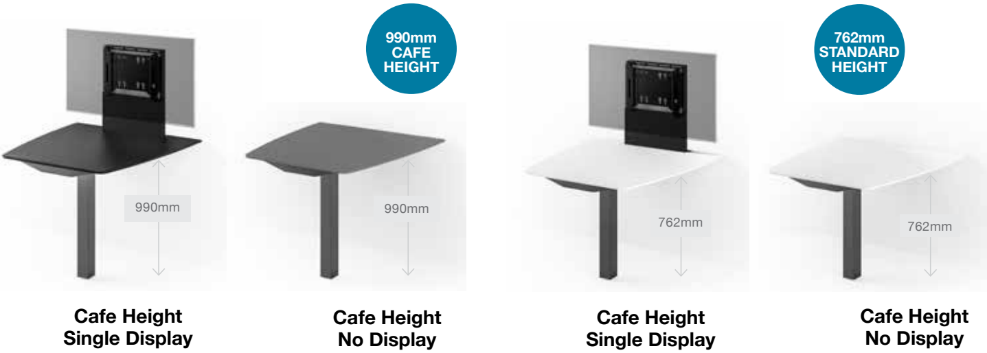
Cafe Table: 1219mm (L) x 1219mm (W) x 990mm (H) 1524mm (L) x 1219mm (W) x 990mm (H)
